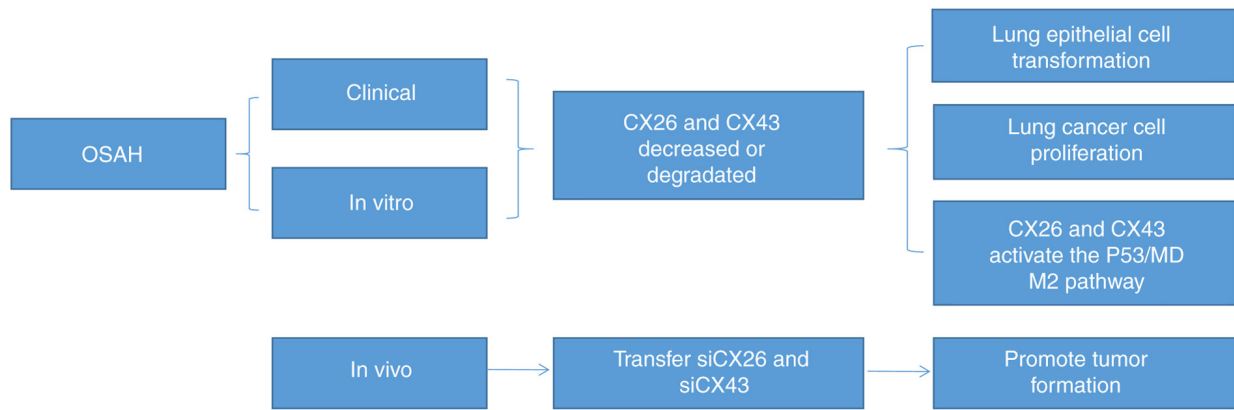
Figure S1. A flow-chart depicting our experimental design. OSAH, obstructive sleep apnea-hypopnea; CX, connexin; MDM2, murine double minute-2; si, small interfering RNA;
