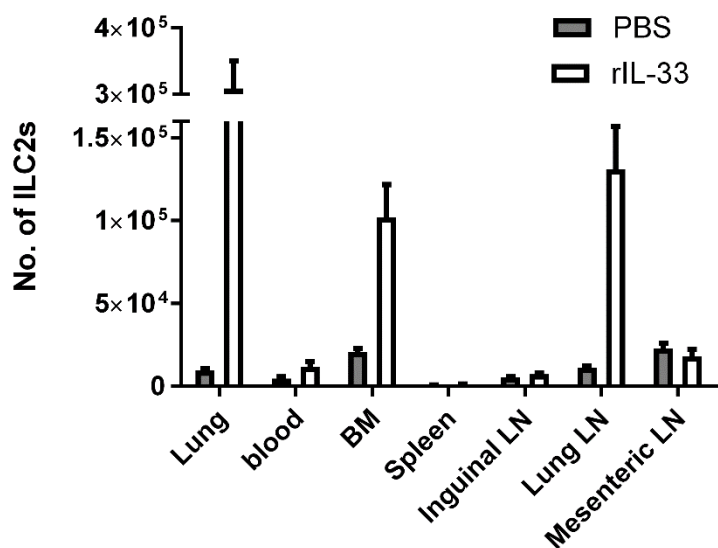
Fig. S2. Quantification of ILC2 in different tissues, related to Fig. 1 A-C. Il13-eGFP mice treated with 3 doses of rIL-33 (1 \mu g per dose) or PBS (25 \mu l) over 1 week and culled 24h after the final dose. ILC2 number in lungs, blood, bone marrow (BM), Spleen, Inguinal lymph node (LN), lung draining LN and mesenteric LN. n \geq 6 mice per group. Data representative of 2 experiments.
