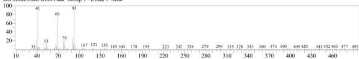
S5 Fig. EI/MS spectrum of compound (5) identified as \beta -Myrcene in the essential oils of M. alternifolia and R. officinalis
