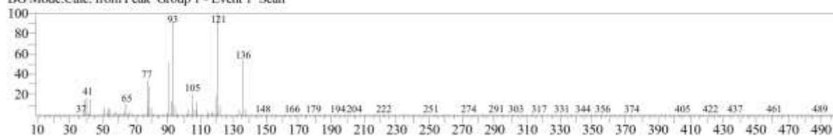
S7 Fig. EI/MS spectrum of compound (7) identified as \alpha -Terpinene in the essential oil of M. alternifolia
