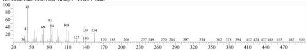
S11 Fig. EI/MS spectrum of compound (11) identified as 1,8-Cineole in the essential oils of M. alternifolia and R. officinalis
