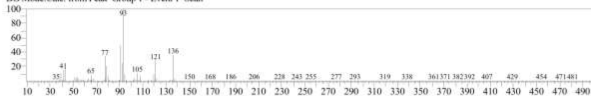
S12 Fig. EI/MS spectrum of compound (12) identified as \gamma -Terpinene in the essential oil of M. alternifolia
