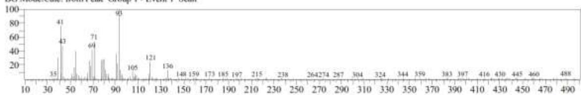
S14 Fig. EI/MS spectrum of compound (14) identified as Linalool in the essential oil of R. officinalis
