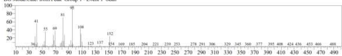
S15 Fig. EI/MS spectrum of compound (15) identified as Camphor in the essential oil of R. officinalis
