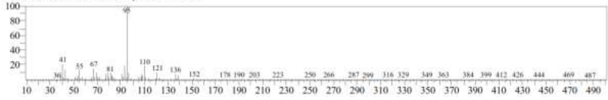
S16 Fig. EI/MS spectrum of compound (16) identified as Borneol in the essential oil of R. officinalis
