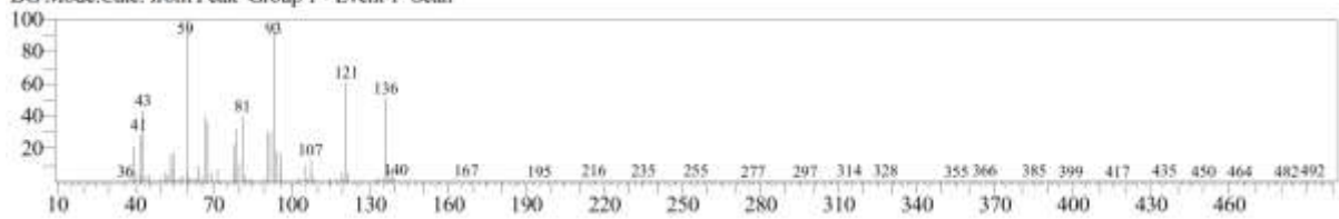
S18 Fig. EI/MS spectrum of compound (18) identified as \alpha -Terpineol in the essential oils of M. alternifolia and R. officinalis
