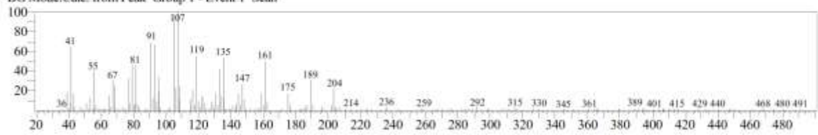
S21 Fig. EI/MS spectrum of compound (21) identified as Ledene in the essential oil of M. alternifolia
