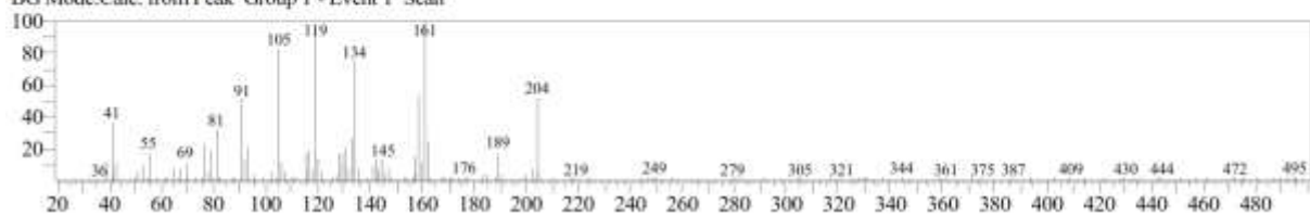
S22 Fig. EI/MS spectrum of compound (22) identified as \delta -Cadinene in the essential oil of M. alternifolia
