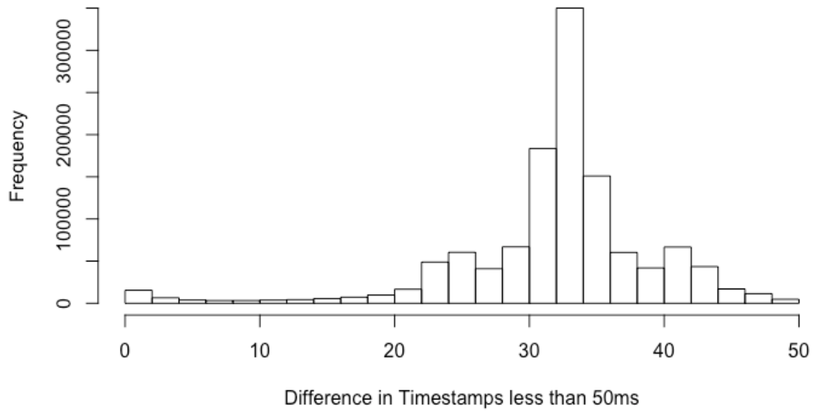
Time Differene in Timestamps for All Participants
