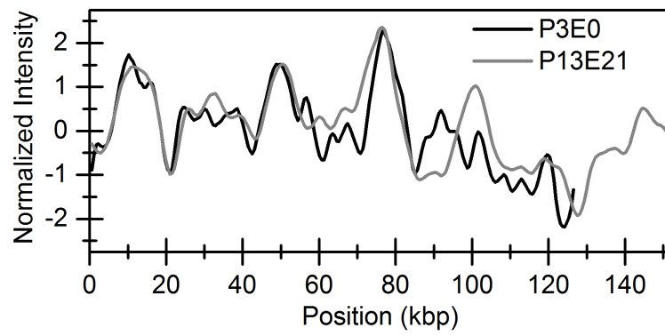
Figure S5. Similarity plot for 130 kbp plasmid in P3E0 and 152 kbp plasmid in P13E21.
