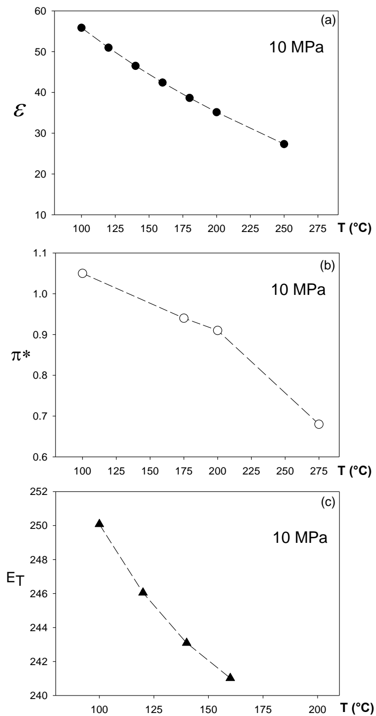
Figure S1. Water polarity expressed as dielectric constant ( \epsilon ), polarity/polarizability ( \pi^* ) and Reichardt's scale ( E_T ) at pressure constant (10 MPa).
