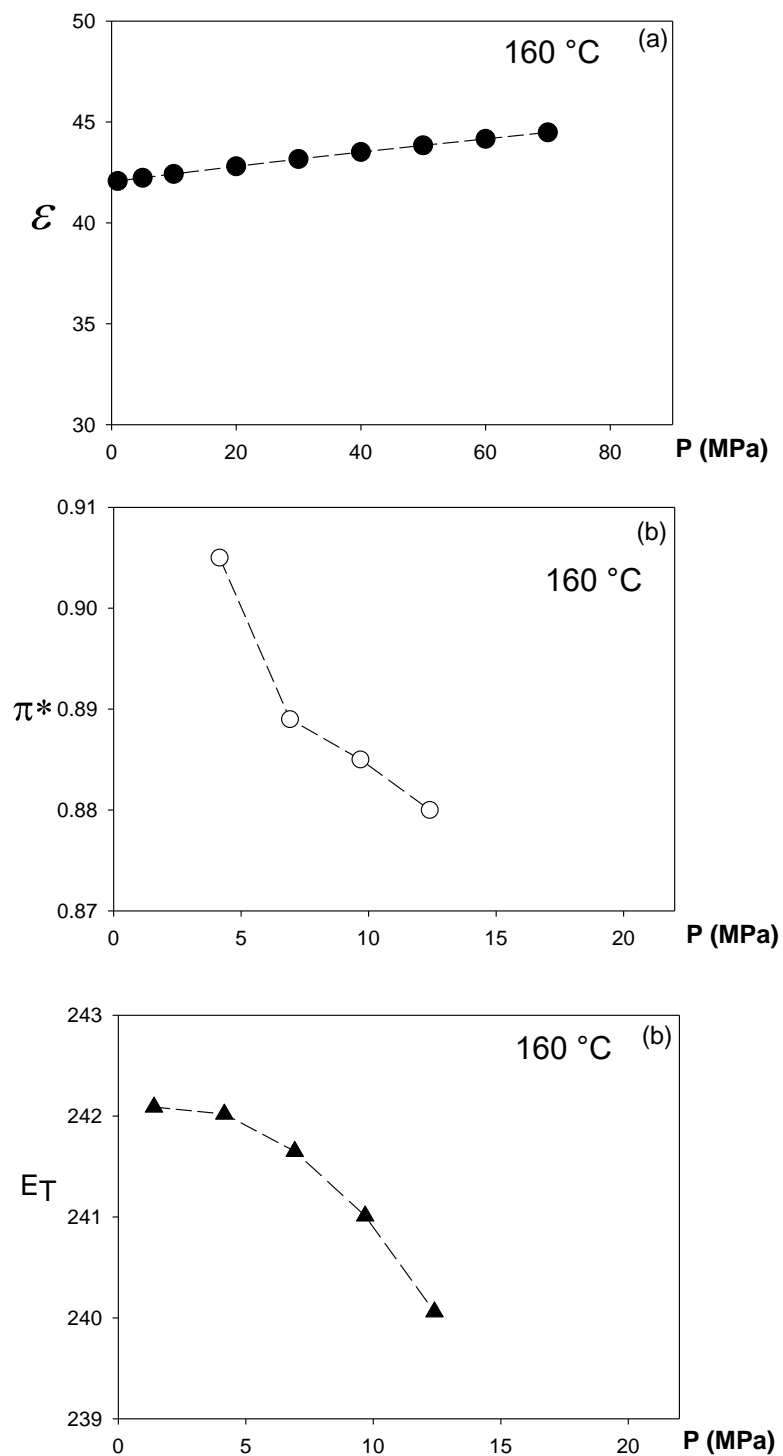
Figure S2. Water polarity expressed as dielectric constant ( \epsilon ), polarity/polarizability ( \pi^* ) and Reichardt's scale ( E_T ) at temperature constant (160°C).
