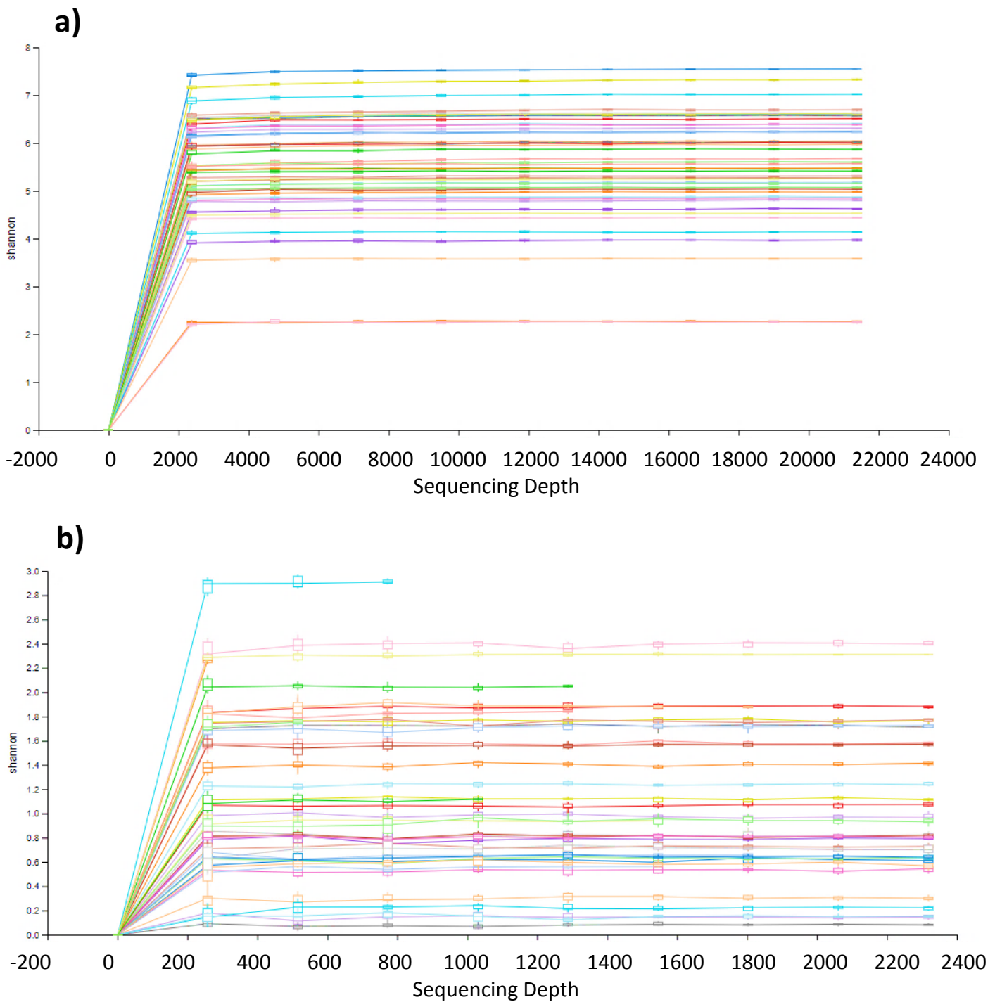
S1 Figure. Rarefaction plots based on Shannon's phylogenetic alpha diversity index for (a) 16S rRNA sequence data and (b) 18S rRNA sequence data (after filtering out contaminating bacterial sequences).
