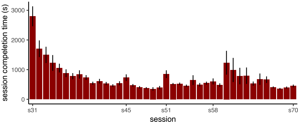
Figure S2. The graph shows the average session duration (across subjects). The animals could earn maximum of 60 outcomes and the session ended as soon as animals earned 60 outcomes. The session length was limited to an hour. The results are for the experiment reported in the main paper. Error-bars represent 1SEM.
