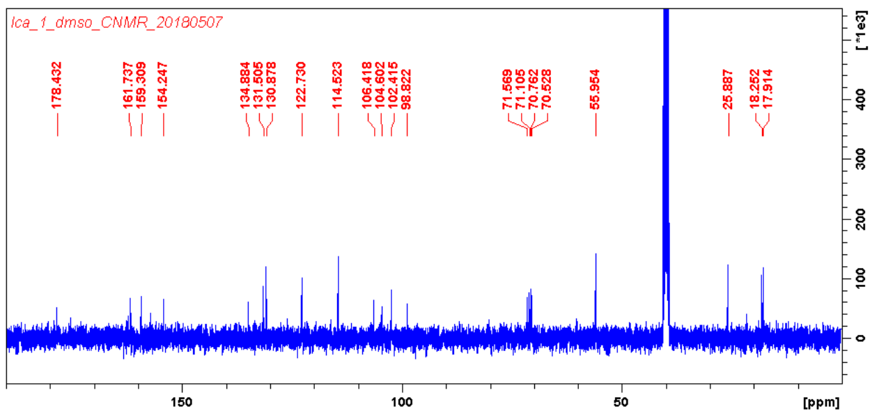
S1-C Fig. Characterization of compound 1, ^{13}\text{C} NMR (100 MHz, \text{DMSO-}d_6 ) spectrum of compound 1.
