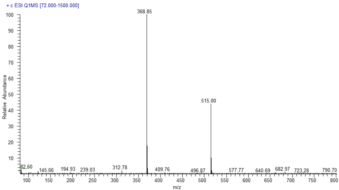
S1-A Fig. Characterization of compound 1, MS/MS spectrum of compound 1.
