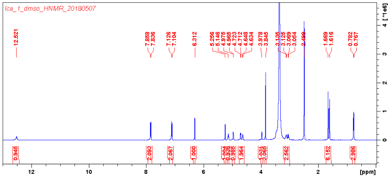
S1-B Fig. Characterization of compound 1, 1 H NMR (400 MHz, DMSO-d 6 ) spectrum of compound 1.
