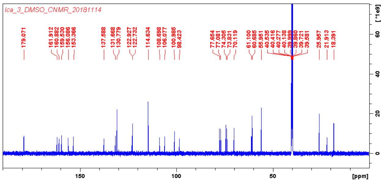
S3-C Fig. Characterization of compound 3, ^{13}\text{C} NMR (100 MHz, \text{DMSO-}d_6 ) spectrum of compound 3.
