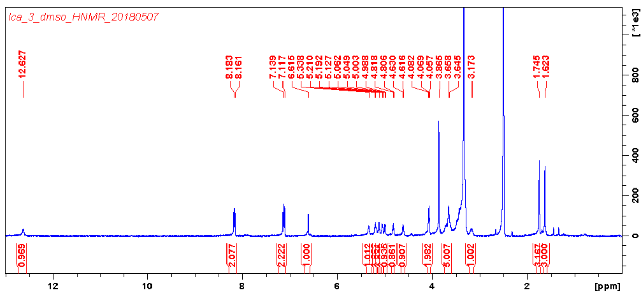
S3-B Fig. Characterization of compound 3, 1 H NMR (400 MHz, DMSO- d 6 ) spectrum of compound 3.
