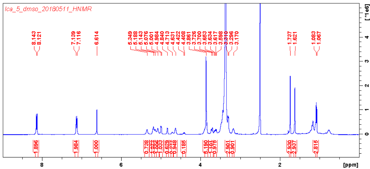
S5-B Fig. Characterization of compound 5, ^1\text{H} NMR (400 MHz, \text{DMSO-}d_6 ) spectrum of compound 5.
