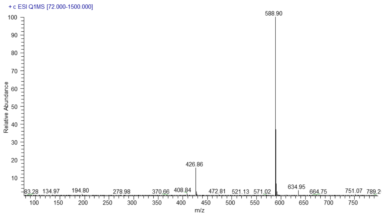
S5-A Fig. Characterization of compound 5, MS/MS spectrum of compound 5.
