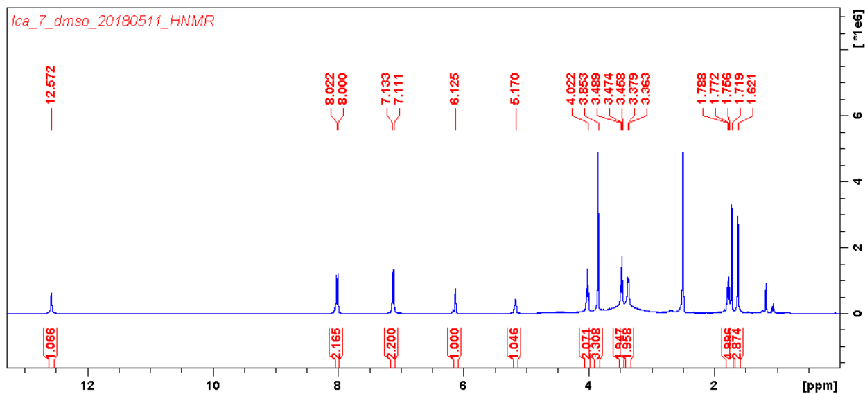
S7-B Fig. Characterization of compound 7, ^1\text{H} NMR (400 MHz, \text{DMSO-}d_6 ) spectrum of compound 7.
