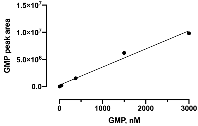
S13Fig. A representative GMP calibration curve measured using HPLC-UV-MS as described in the Methods section. GMP standard concentrations used were 5.9, 47, 375, 1500, and 3000 nM.
