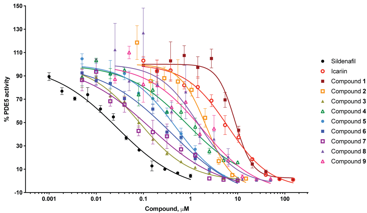
S14 Fig. Dose-response curve and best-fit line as determined by nonlinear regression analysis for each icariin analog and sildenafil in in vitro PDE5 inhibition assays. Each data point represents the mean (from at least three replicates) \pm SEM. Solid lines represent the best-fit line as determined by nonlinear regression analysis.
