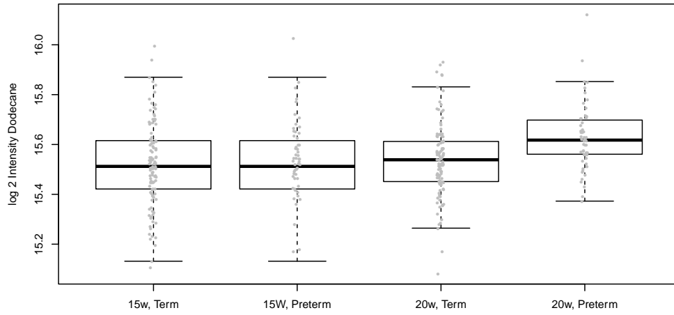
Dodecane Intensity at 15, 20 weeks
