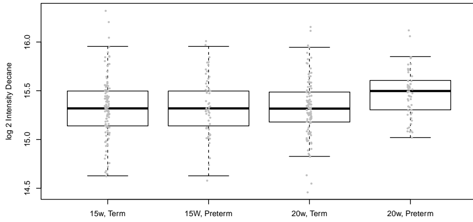
Decane Intensity at 15, 20 weeks
