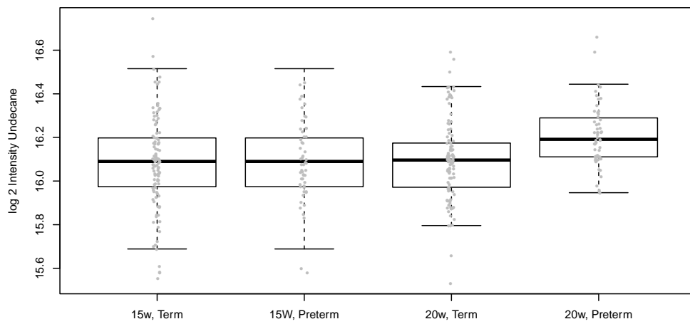
Undecane Intensity at 15, 20 weeks
