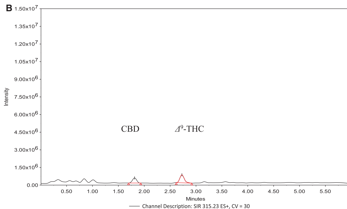
SUPPLEMENTARY FIG. S1. Representative mass chromatograms for cultivar 1 extract using UAE: (A) ESI (-ve) mode for detection of acidic phytocannabinoids, and (B) ESI (+ve) mode for detection of neutral phytocannabinoids. ESI, electron spray ionization; UAE, ultrasound-assisted extraction.
