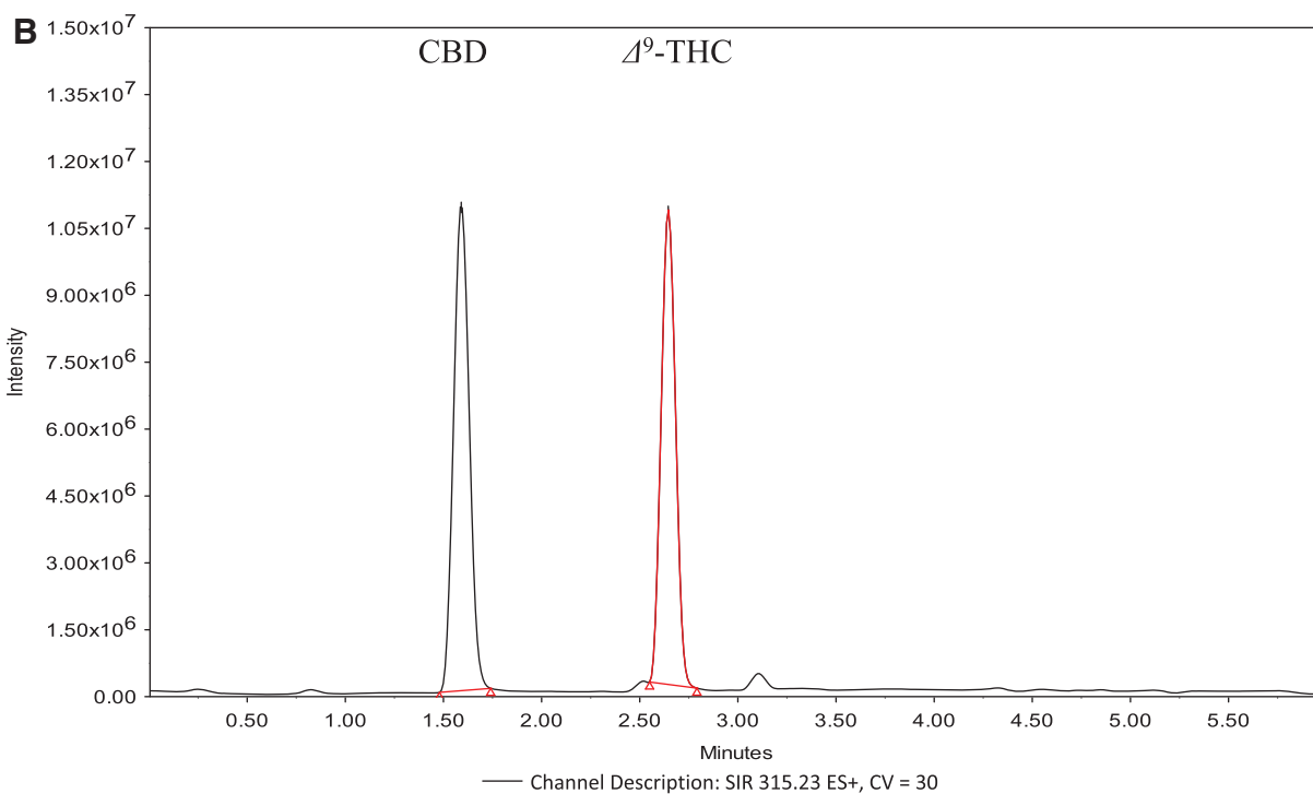
SUPPLEMENTARY FIG. S2. Representative mass chromatograms for cultivar 1 extract using MAE. (A) ESI (-ve) mode for detection of acidic phytocannabinoids and (B) ESI (+ve) mode for detection of neutral phytocannabinoids. MAE, microwave-assisted extraction.
