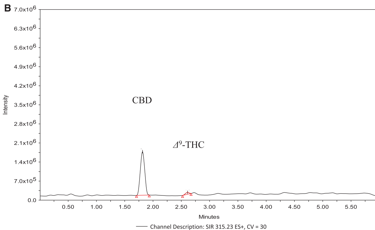
SUPPLEMENTARY FIG. S3. Representative mass chromatograms for cultivar 2 extract using UAE. (A) ESI (-ve) mode for detection of acidic phytocannabinoids and (B) ESI (+ve) mode for detection of neutral phytocannabinoids.
