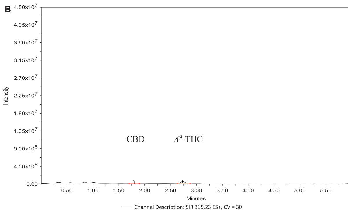
SUPPLEMENTARY FIG. S5. Representative mass chromatograms for cultivar 3 extract using UAE. (A) ESI (-ve) mode for detection of acidic phytocannabinoids and (B) ESI (+ve) mode for detection of neutral phytocannabinoids.
