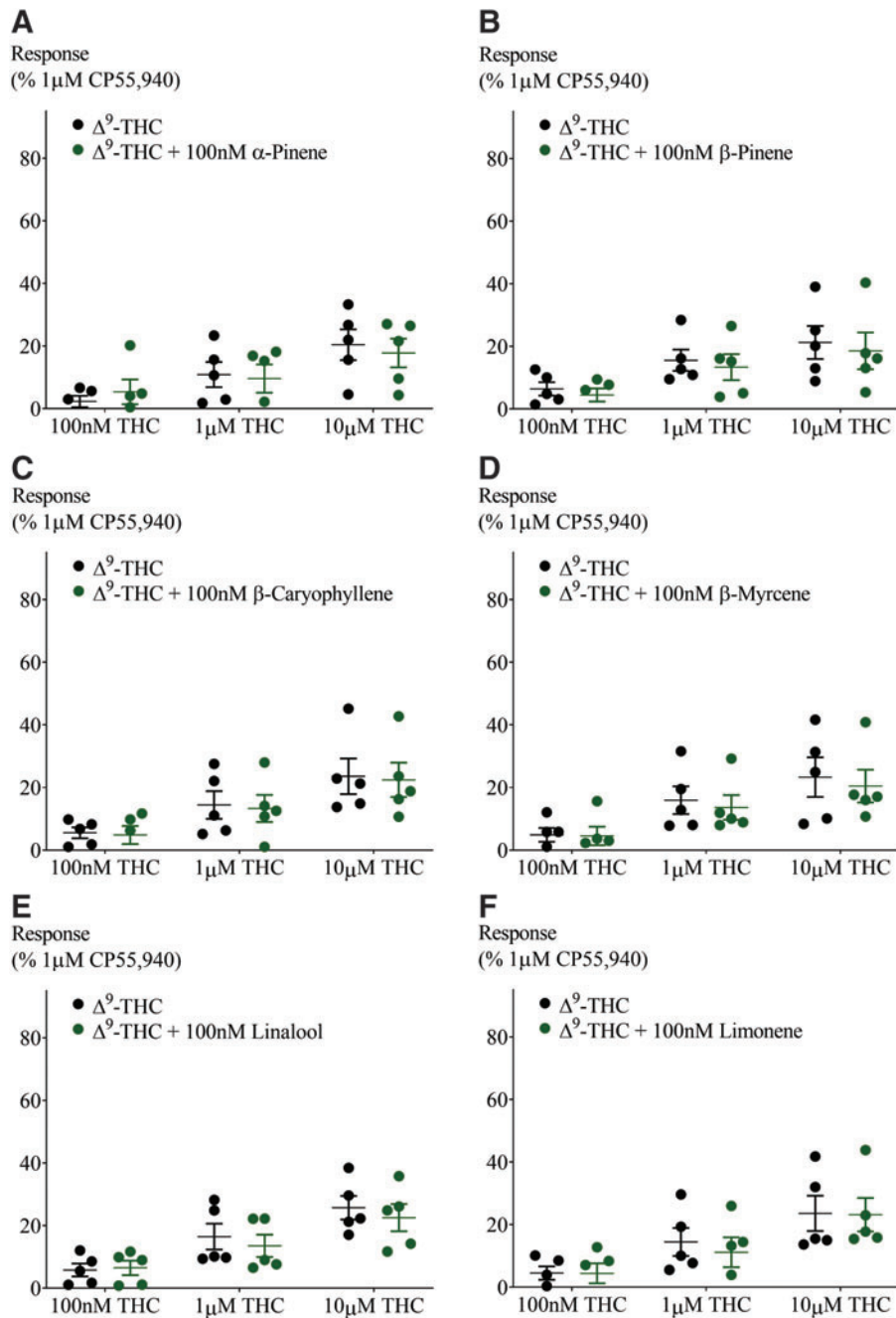
SUPPLEMENTARY FIG. S3. Effect of 100 nM terpenoids on peak hyperpolarization induced by \Delta^9 -THC in AtT20-CB 2 cells. Terpenoids tested were (A) \alpha -pinene, (B) \beta -pinene, (C) \beta -caryophyllene, (D) \beta -myrcene, (E) linalool, and (F) limonene. Response to \Delta^9 -THC at two submaximal and one maximal concentration ( n=5 , SEM, unpaired t -test p > 0.50 ). Data presented as % of maximum CP55,940 (1 \mu M) response.
