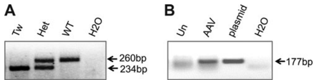
Supplementary Fig. S1. PCR genotyping of experimental mice and PCR confirmation of AAV injected twitcher mice. (A) Representative PCR photomicrograph of genotyping results. (B) Representative PCR photomicrograph of AAV injection validation. Tw, twitcher mouse; Het, heterozygous mouse; WT, wild type mouse; H2O, negative control (without genome DNA); Un, un-injected twitcher mouse; AAV, AAV injected twitcher mouse; Plasmid, positive control using the cis-plasmid pXP46 as the PCR template; H2O, negative control.
