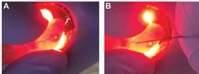
Supplementary Fig. S2. Systemic injection of the AAV vector via the facial vein in a 2-day-old twitcher mouse. (A) Identification of the facial vein using the Wee-sight transilluminator vein finder. (B) Delivery of the AAV vector from the facial vein.
