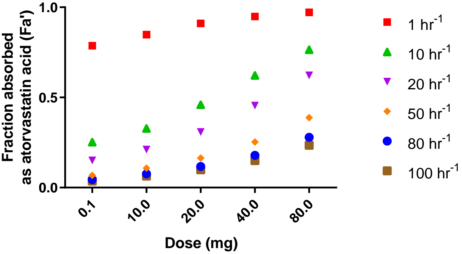
Figure S1. Sensitivity analysis on the effect of stomach degradation/lactone conversion on A) atorvastatin acid Cmax and B) fraction absorbed as atorvastatin acid (Fa'). Degradation rate constant included in the model is 50 hr -1 . Sensitivity analysis was performed with a population representative.
