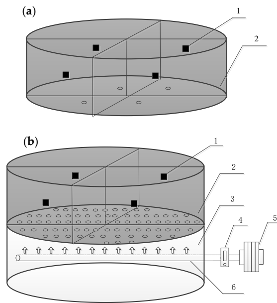
Figure S1. (a) Schematic diagram of composting reactors for farmer compost, anaerobic compost and mixed compost; (b) Schematic diagram of composting reactors for aerobic compost; 1—temperature sensor; 2—Pile layer; 3—Air distribution layer; 4—Rotameter; 5—Air pump; 6—Air distributor.
