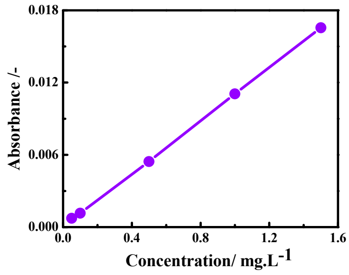
Figure S1. UV-Visible calibration curve of AB40.
