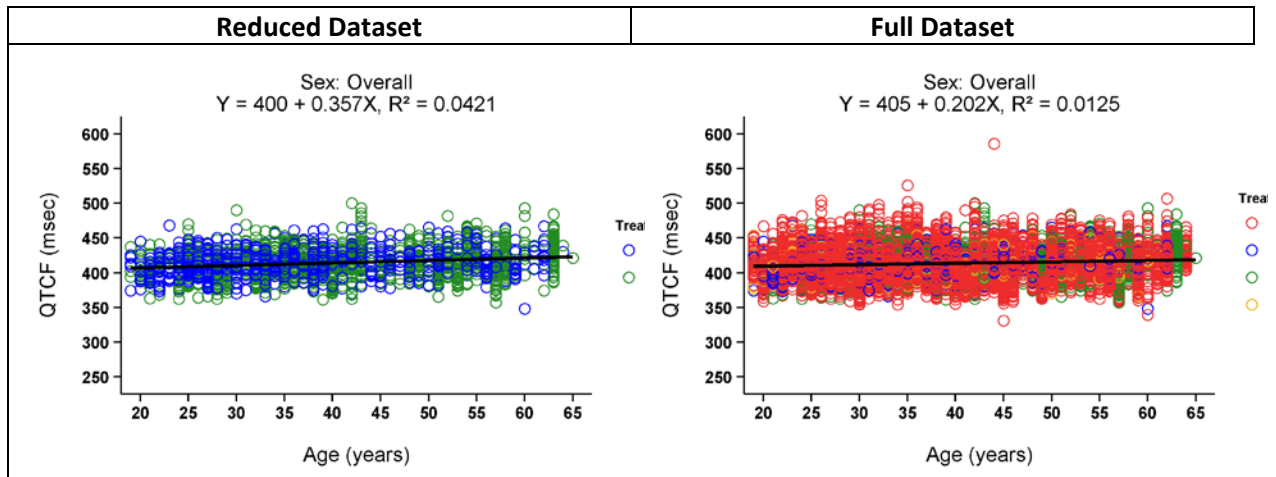
Figure S4: Relationship between Age and QTcF Intervals
