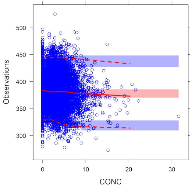
Figure S3: Visual Predictive Check: QTc by Concentration
