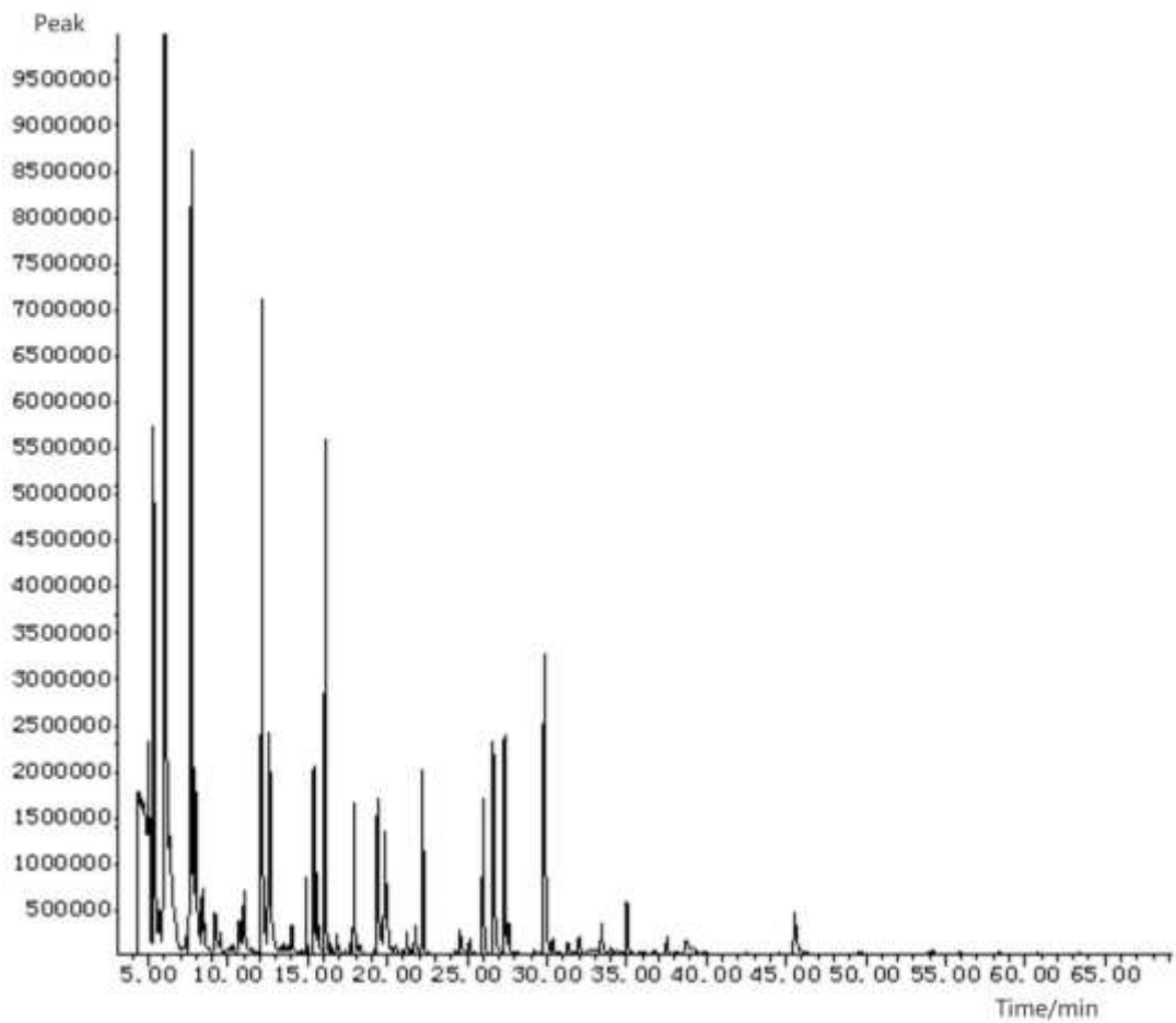
Fig 2. GC-MS chromatograms (T2 sample)
