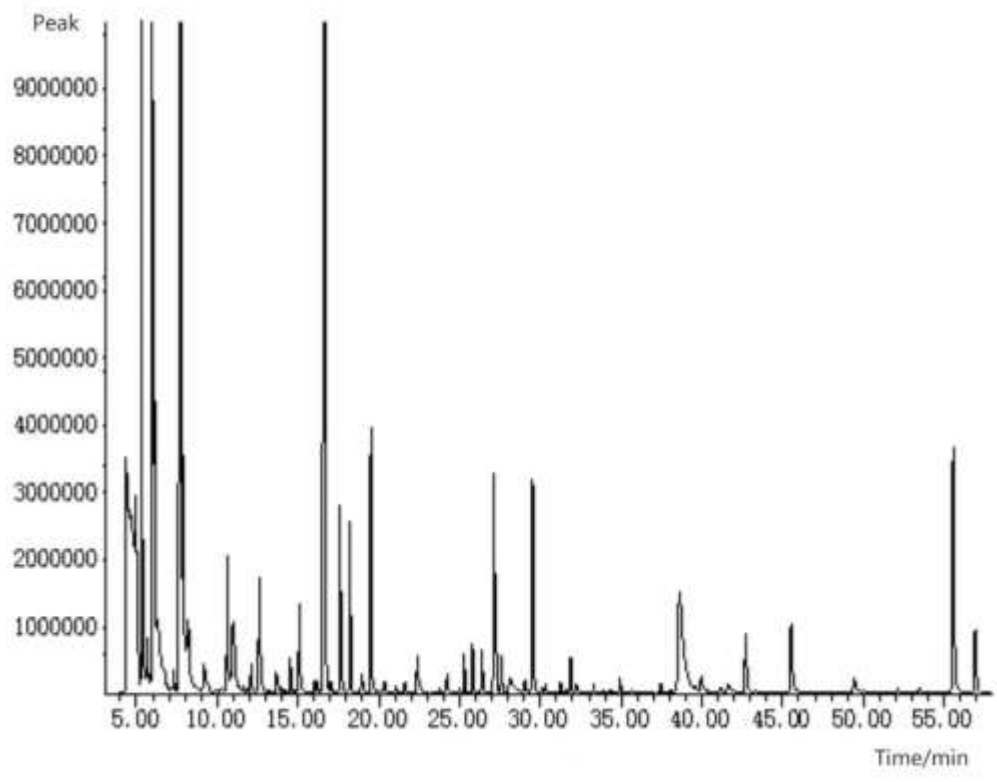
Fig 3. GC-MS chromatograms (T3 sample)
