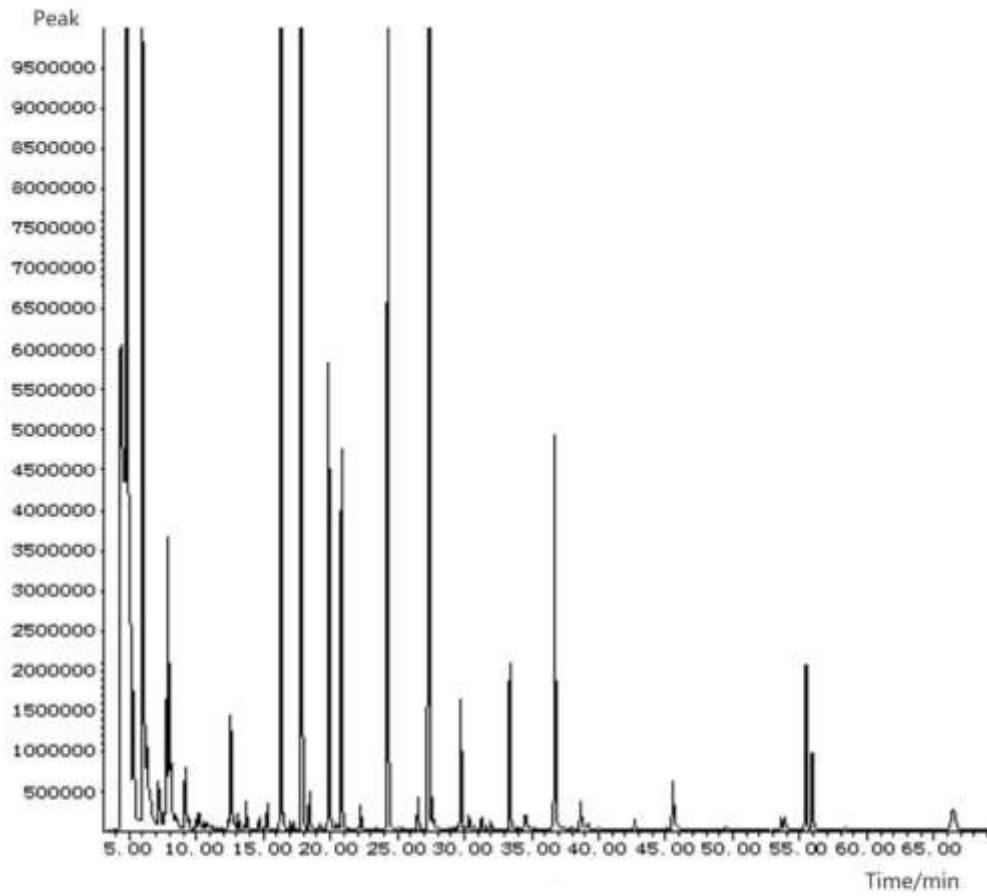
Fig 1. GC-MS chromatograms (T1 sample)
