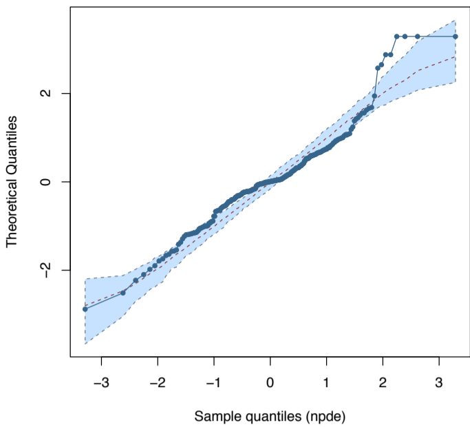
Q-Q plot versus N(0,1) for npde
