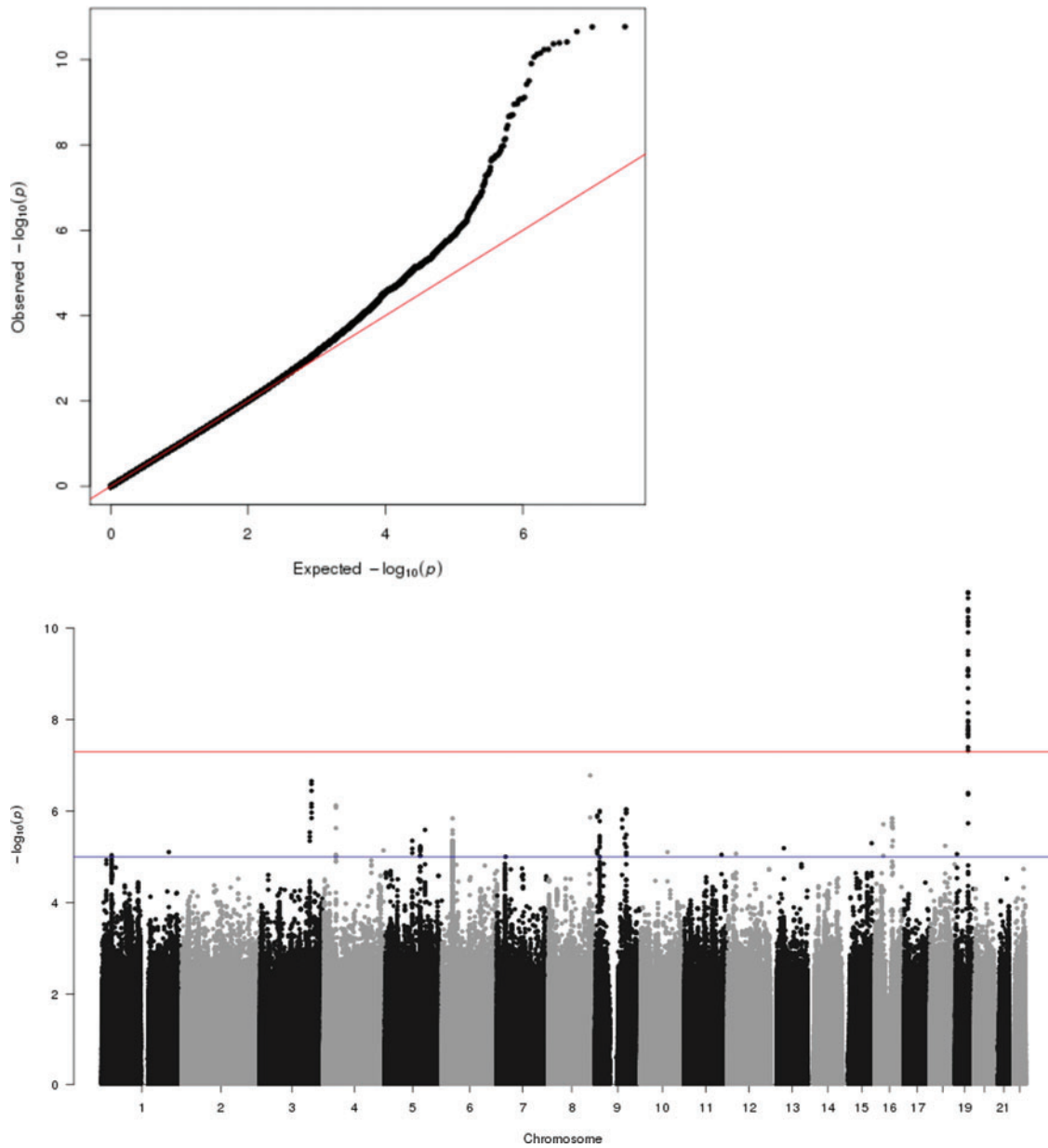
SUPPLEMENTARY FIG. S2. QQ plot and GWAS of \log_{10}(\text{PTVL}) . GWAS, genome-wide association study; QQ, quantile-quantile.
