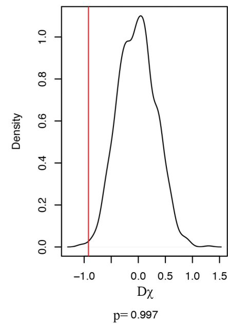
F. Euler Characteristic
