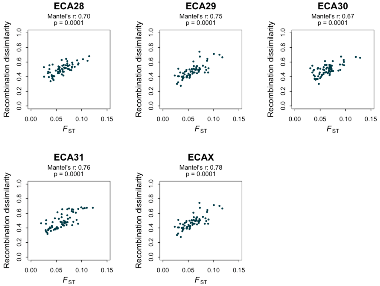
Supplemental Figure S3. Pairwise recombination dissimilarity vs. F_{ST} by chromosome. Recombination dissimilarity is 1 - \text{Spearman's rank correlation coefficient} for recombination rates across the chromosome. Above each plot is the results of the Mantel test for matrix correlation.
