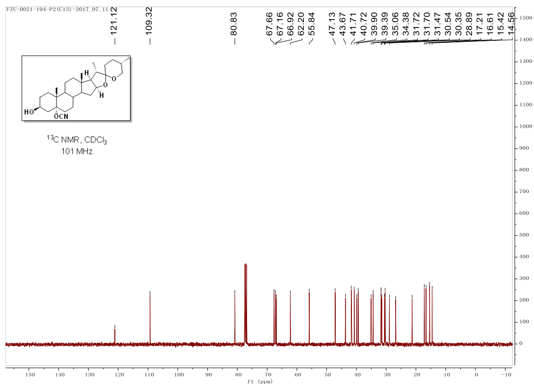
Figure S2: ^{13}\text{C NMR} spectrum of P2.
