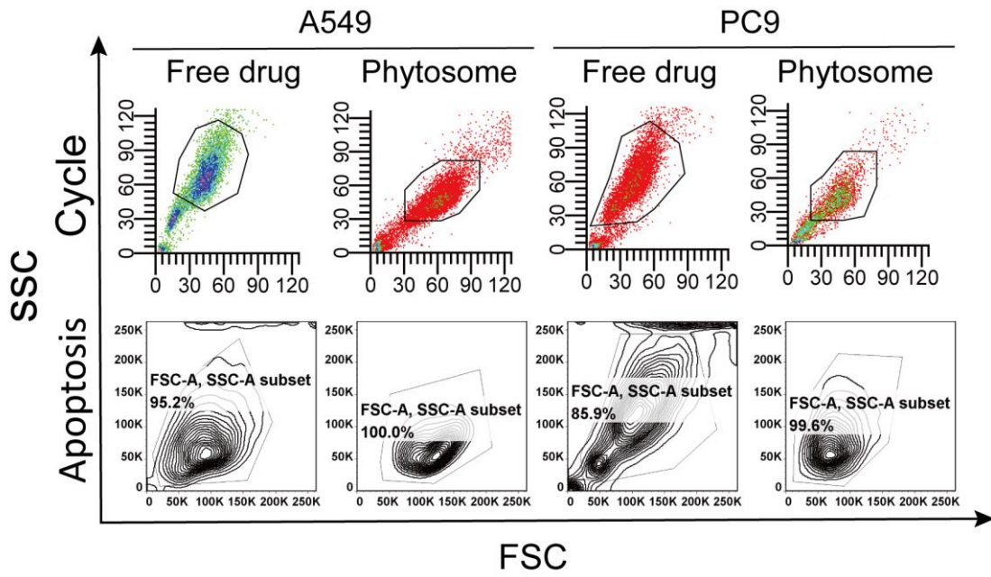
Figure S3: The gating for flow cytometry.
