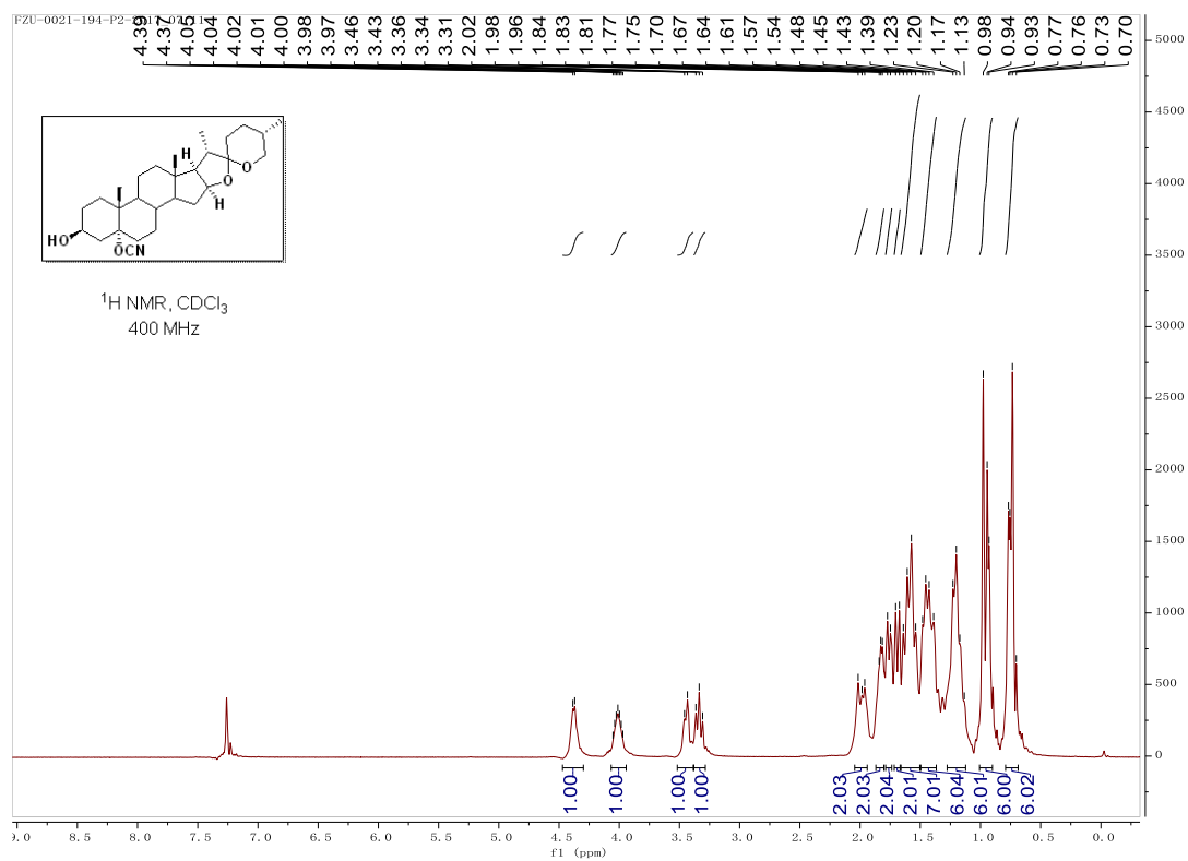
Figure S1: ^1\text{H NMR} spectrum of P2.
