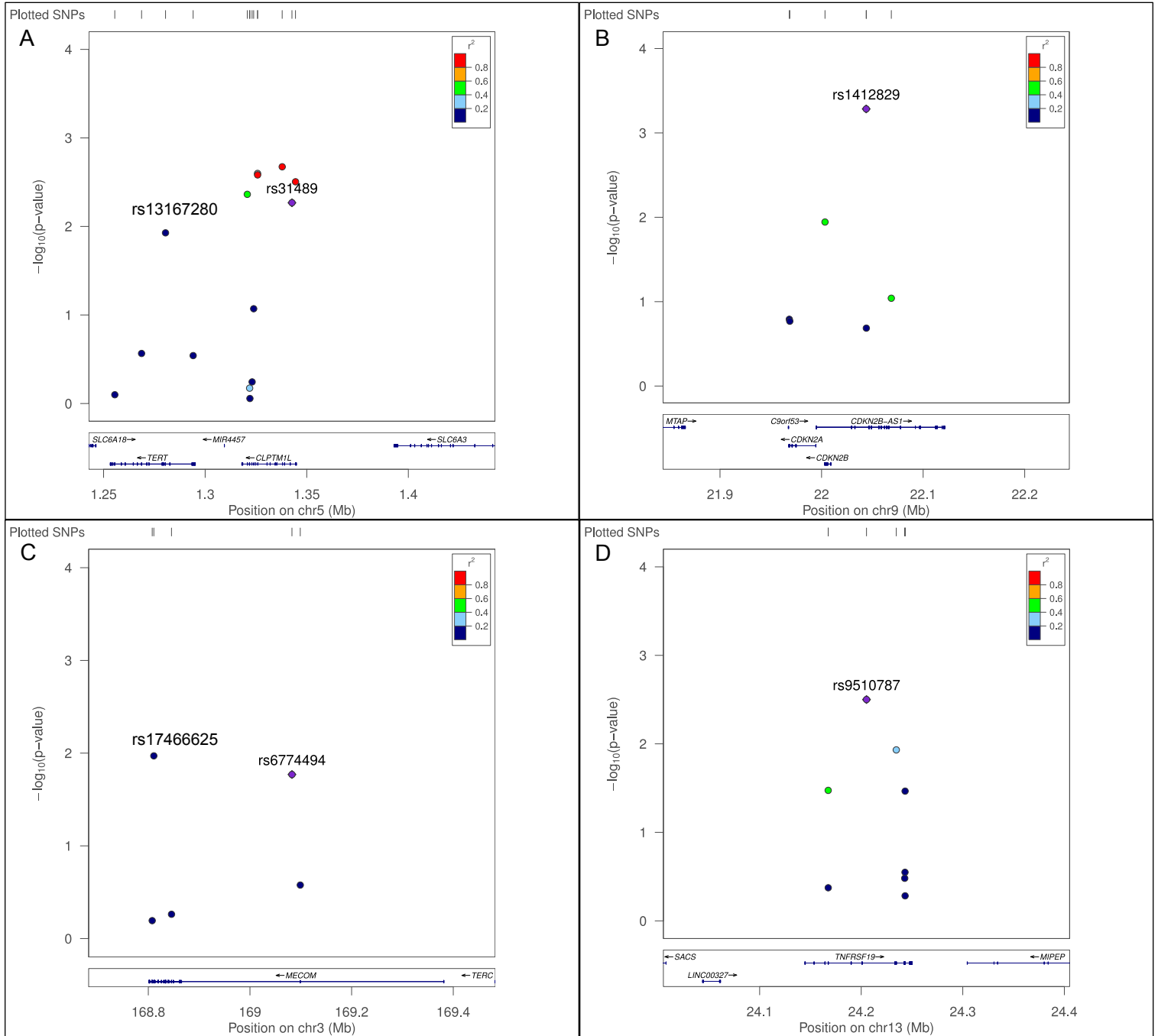
Supplementary Figure 1. Regional plot for the A) CLPTM1L/TERT locus, B) CDKN2A/2B locus, C) MECOM locus, D) TNFRSF19 locus.
