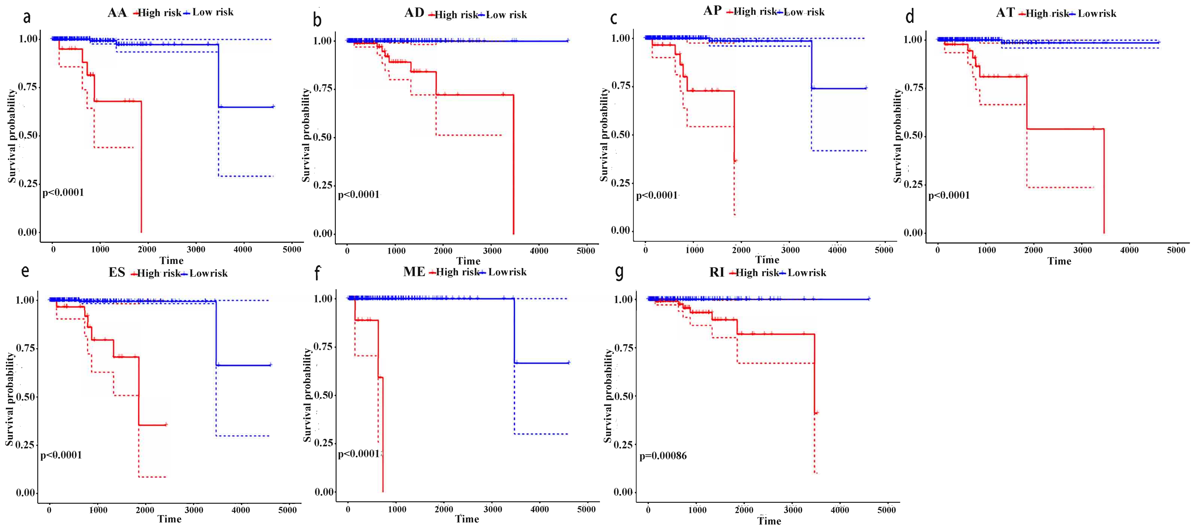
Fig. S1 Kaplan-Meier analysis of top10 OS associated AS events in PCa.
