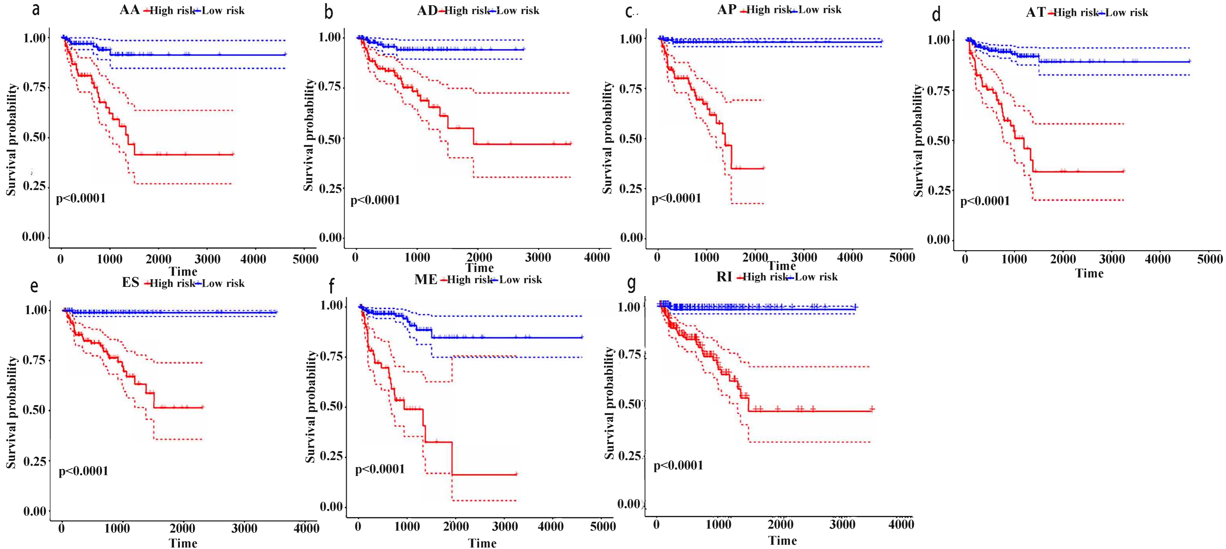
Fig. S2 Kaplan-Meier analysis of top10 RFS associated AS events in PCa.
