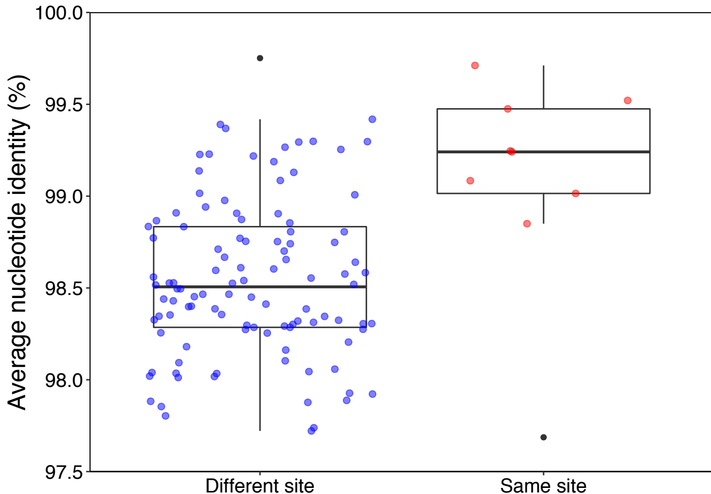
Figure S4 Average nucleotide identity (ANI) comparisons between genomes from the same site (n= 9) and different sites (n= 108) in the Eel River watershed. Boxplots show the median and interquartile range. Whiskers extend 1.5 times the interquartile range, and outlier points are indicated in black. The mean ANI in the same site comparisons was higher than different site comparisons (Mann-Whitney test, p < 0.01 ).
