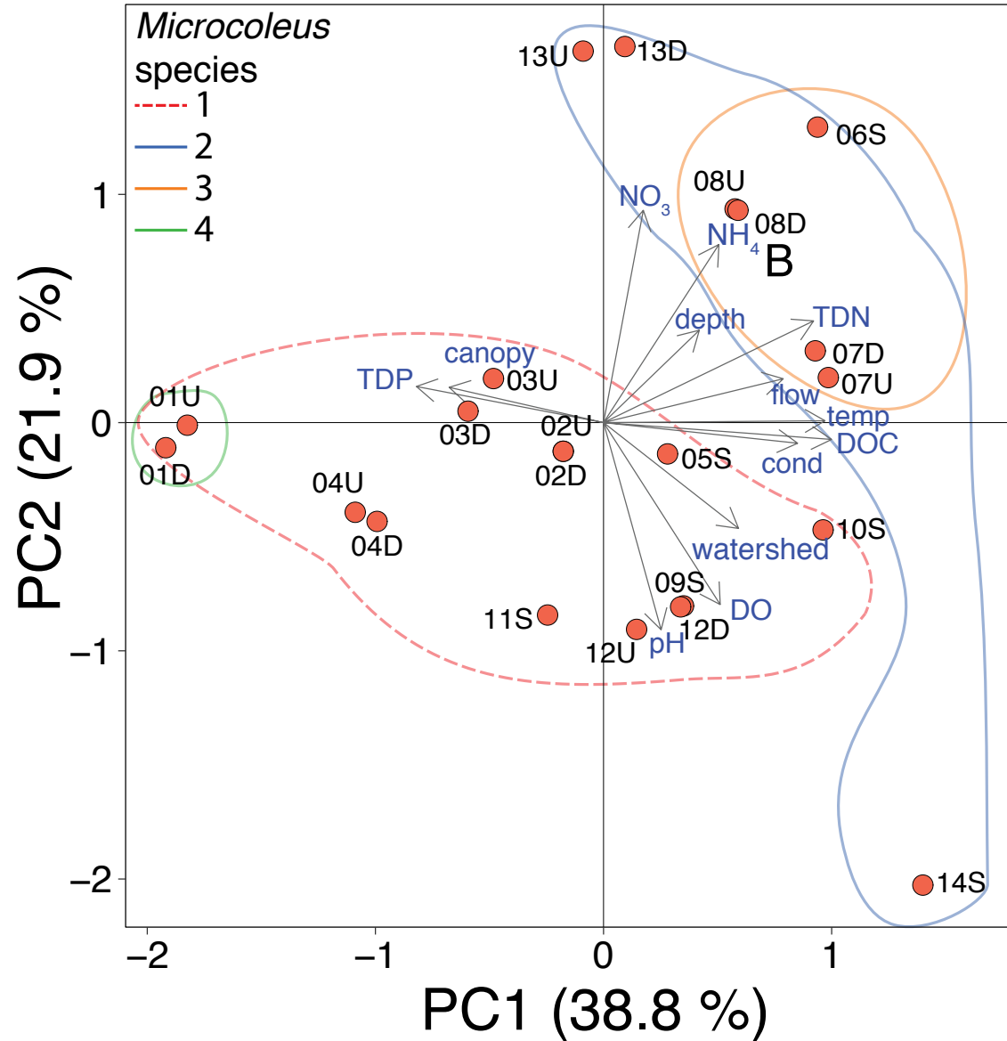
Figure S5 Principal components biplot of environmental conditions at each sampling site. Sites are labeled with red points, and environmental variables labeled with vectors. The percentage of variation described by each axis is written in parentheses. Sites where Microcoleus species 1-4 were found are enclosed by different colored lines for each Microcoleus species. Some samples contained genomes from multiple ANI clusters, and samples 02D and 02U share the same point.
