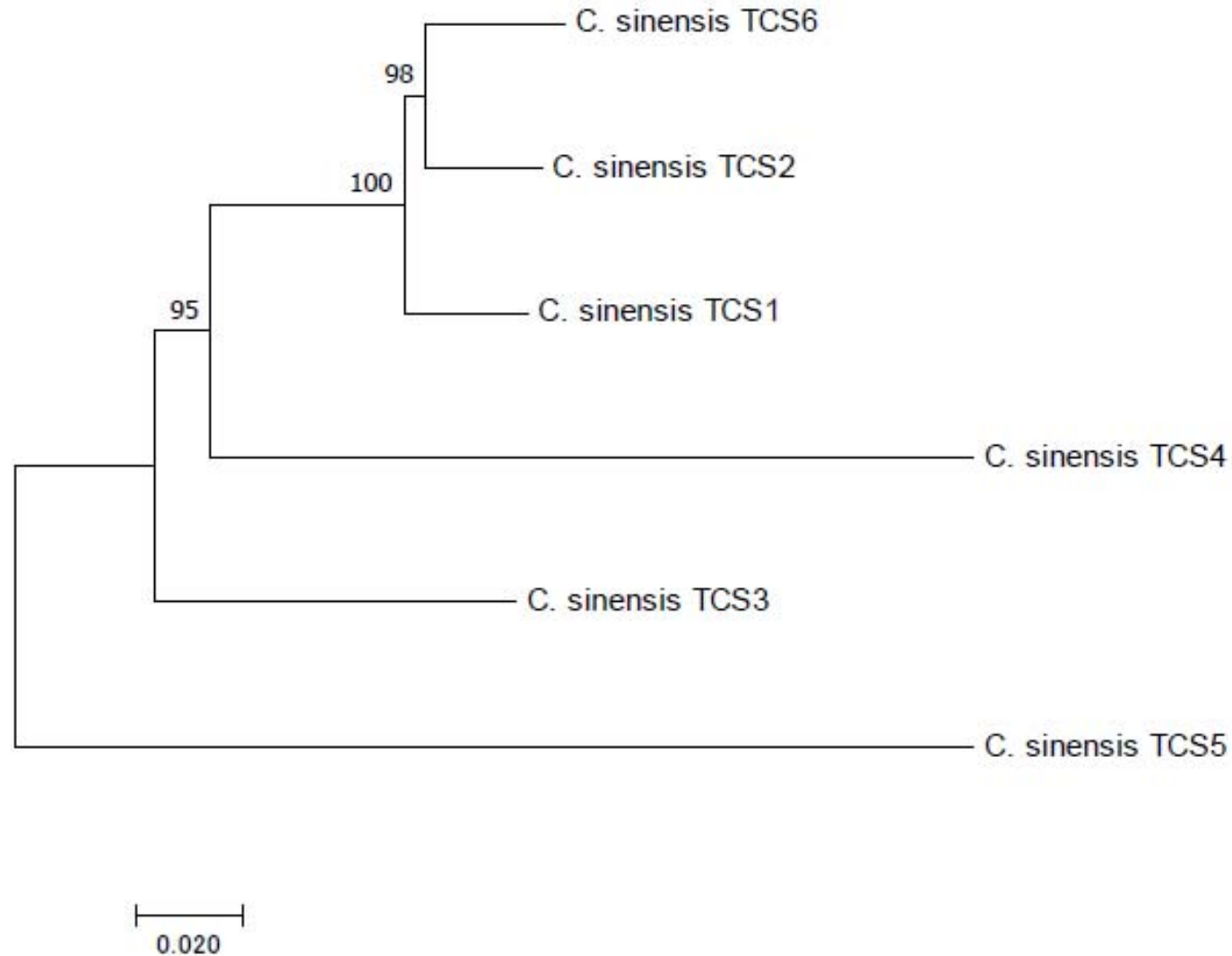
Supplemental Fig. 1 Evolutionary relationships of TCS genes. The evolutionary history was inferred using the Neighbor-Joining method. The percentage of replicate trees in which the associated taxa clustered together in the bootstrap test (500 replicates) are shown next to the branches. Evolutionary analyses were conducted in MEGA7.
