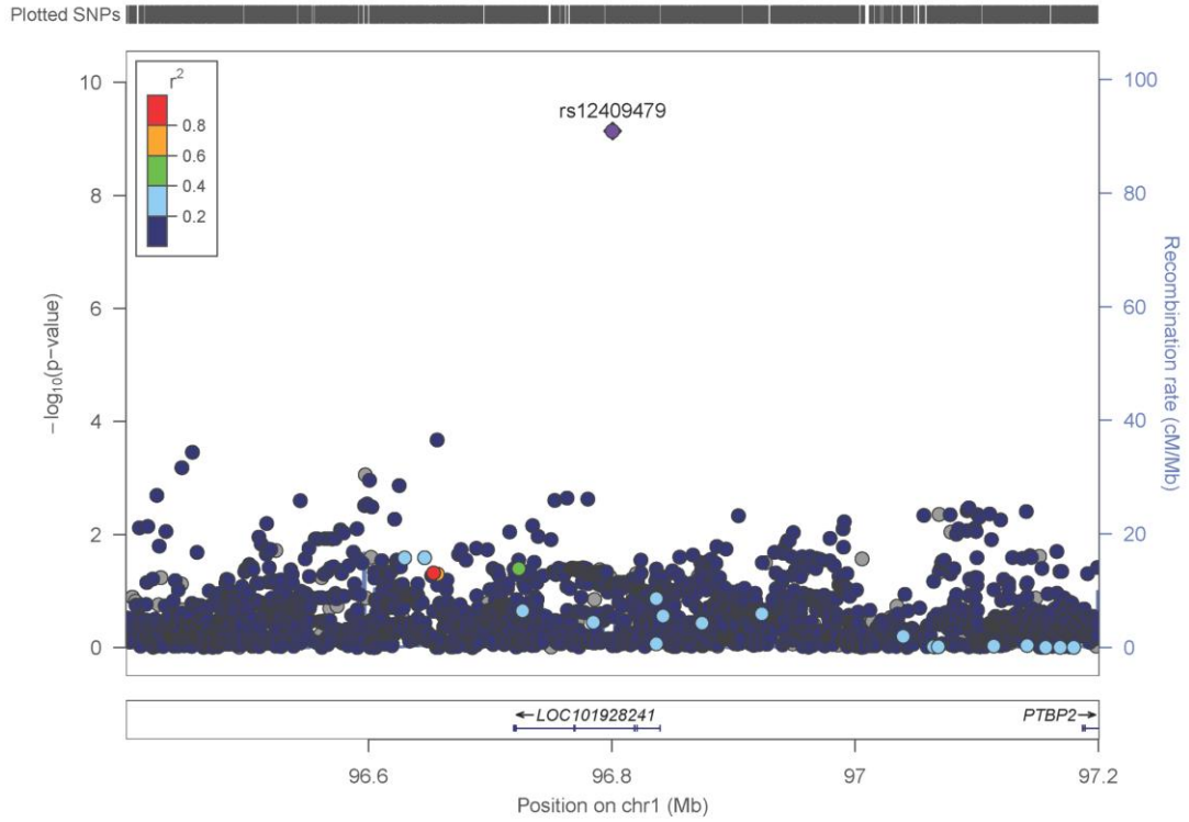
Supplemental Figure 2. Regional plot of rs12409479 .
