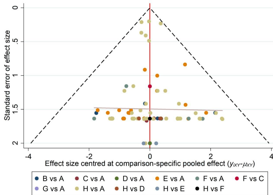
Appendix 9 Comparison-adjusted funnel plot for cancers of digestive system with incretin-based therapies
