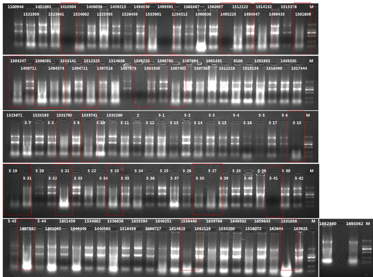
Figure S1. Quality control of the RNA samples for reverse transcription-quantitative polymerase chain reaction validation. The RNA samples were analyzed using agarose gel electrophoresis. The 26 samples that were of low quality are indicated by the red boxes. M, marker.
