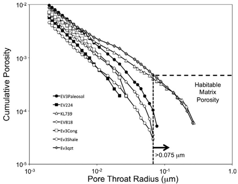
SUPPLEMENTARY FIG. S1. Cumulative porosity in fractional volume versus pore throat radius as measured by Hg porosimetry. Symbols refer to different core samples of sedimentary rock and volcanic rock (KL739) from the Witwatersrand Supergroup. Dashed line demarcates the maximum fractional volume observed for pore diameters greater than 0.15 microns.
