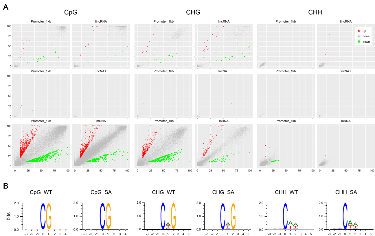
Figure S4. RMCs of transcripts (A) and base composition analysis (B) for CpG, CHG and CHH contexts.
